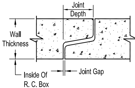
Section thru Box Joint
