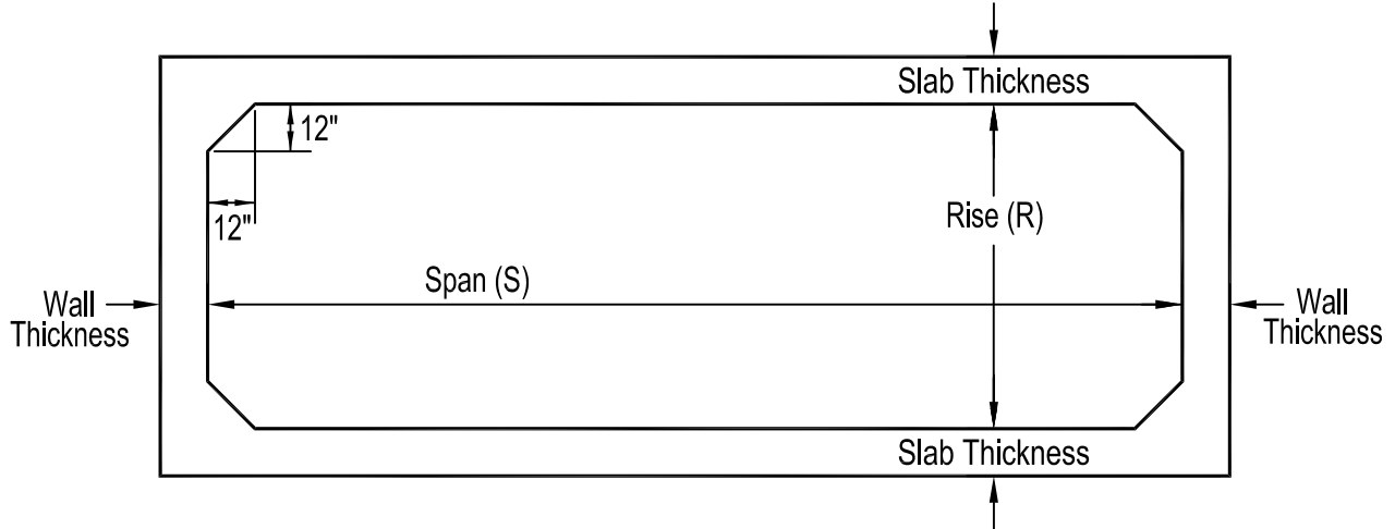
Section thru Box Culvert
