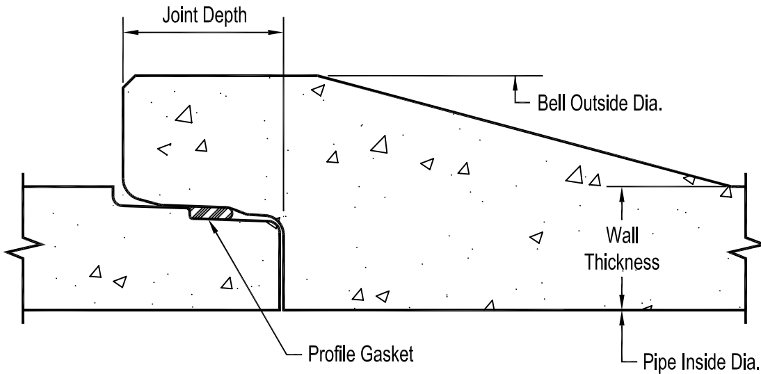
Section Thru Joint
