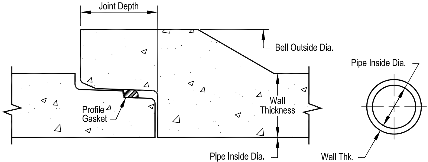
Section Thru Joint
